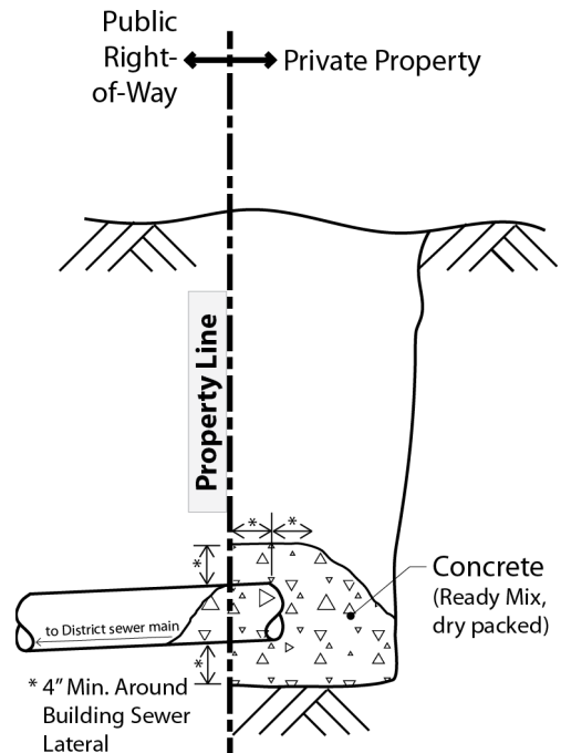
FIGURE 1. Cutting and plugging for permanent disconnection of building sewer lateral.
